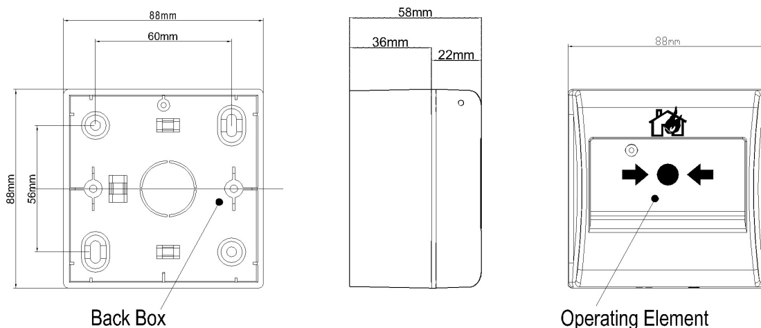
Fig.1 Dimensions
