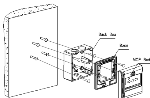
Fig.2 Surface mounting
